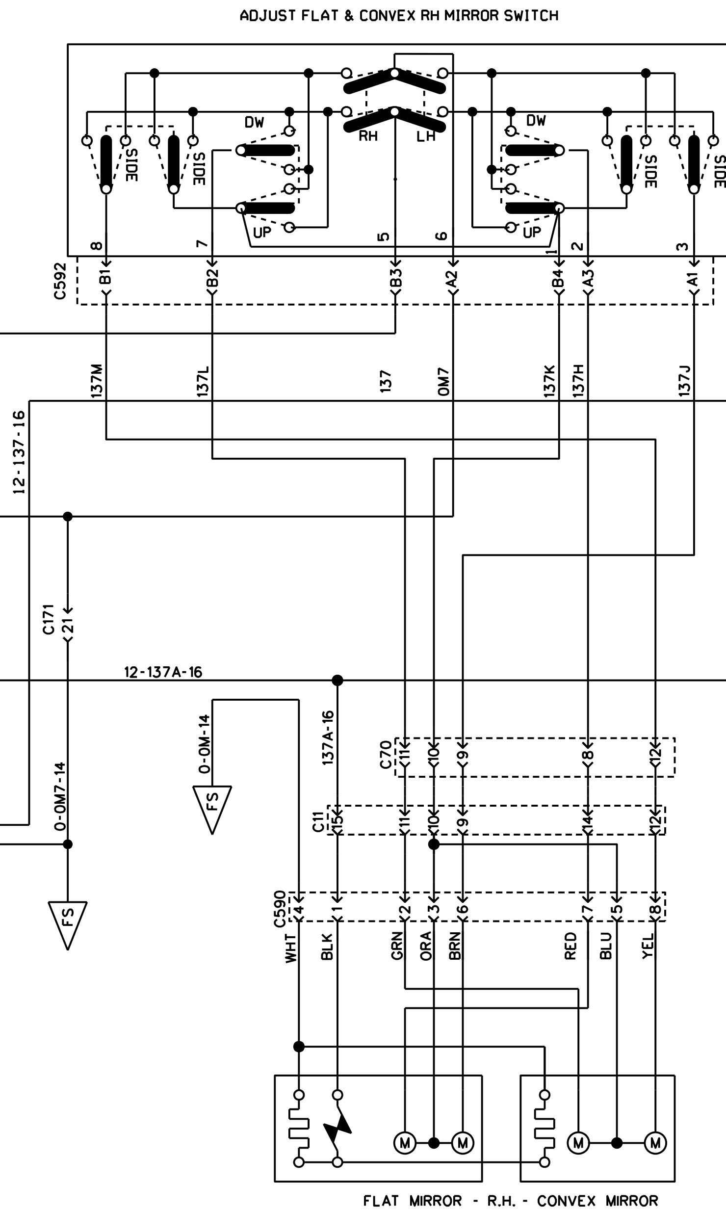
REAR VIEW MIRROR RAMCO FLAT & CONVEX - 2 ADJUSTMENT SW. & 1 HEATED SW.
